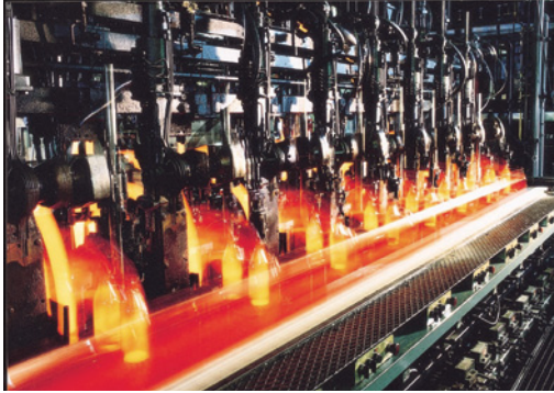
From the molten state through to the cooling process, continuous temperature monitoring ensures that glass retains its properties as it travels through the manufacturing process.
